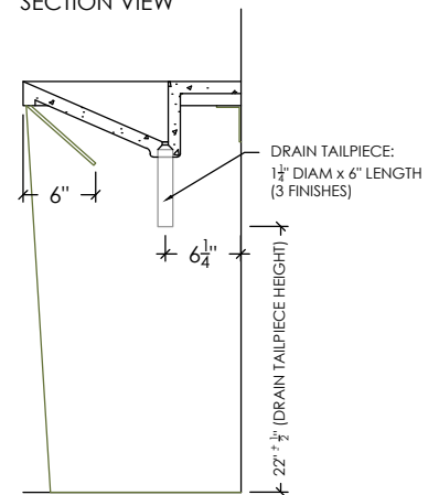
SECTION VIEW
