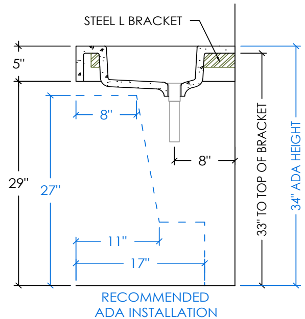
RIGHT SECTION
