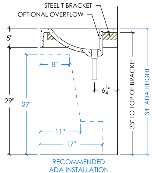
RIGHT SECTION
