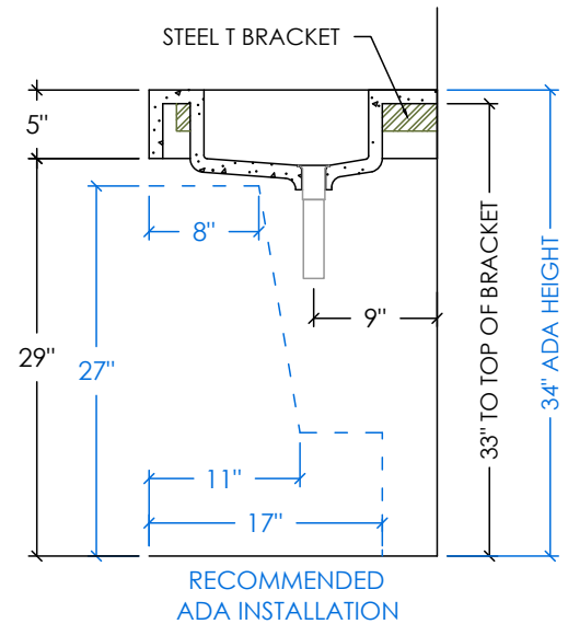
RIGHT SECTION
