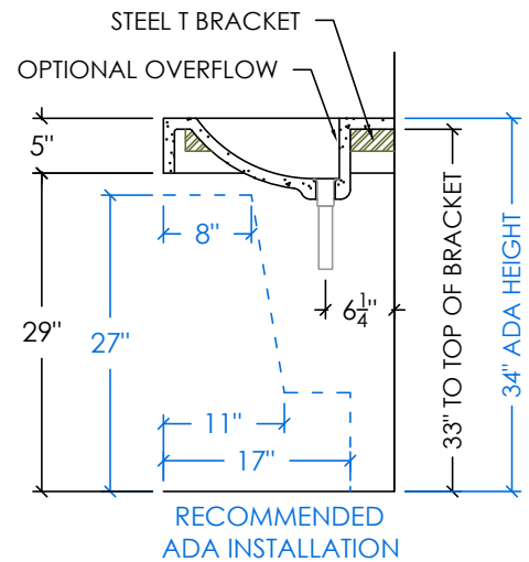
RIGHT SECTION
