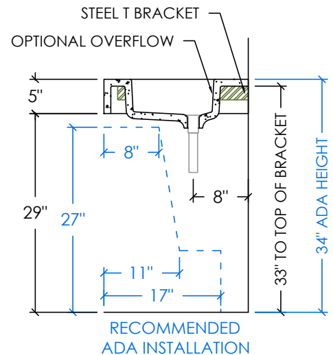
RIGHT SECTION
