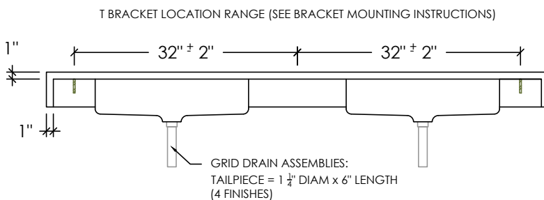
REAR ELEVATION
