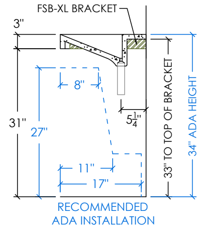
RIGHT SECTION
