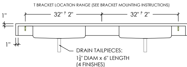
REAR ELEVATION
