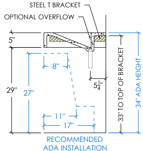
RIGHT SECTION
