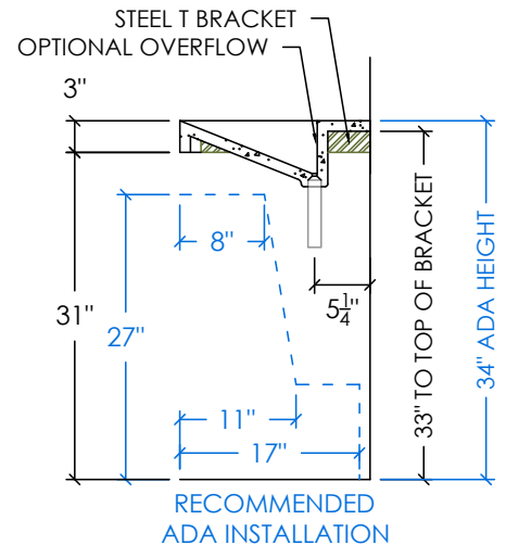
RIGHT SECTION
