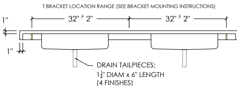
REAR ELEVATION
