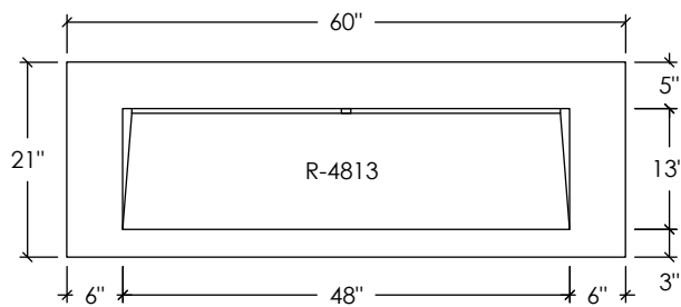
PLAN VIEW
