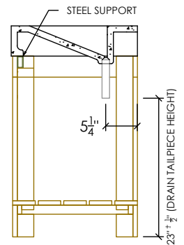
SECTION VIEW
