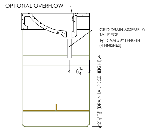
SECTION VIEW
