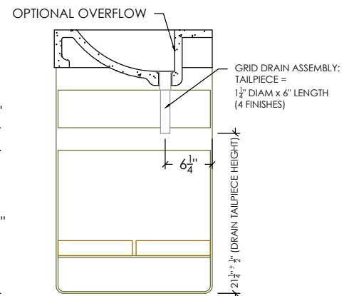
SECTION VIEW
