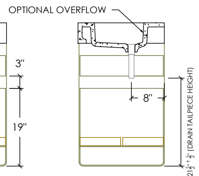
SECTION VIEW
