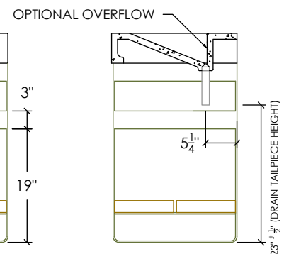
SECTION VIEW
