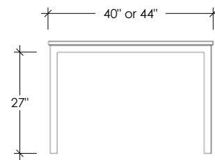
SIDE ELEVATION
