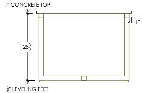
SIDE SECTION
