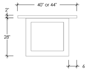
SIDE ELEVATION
