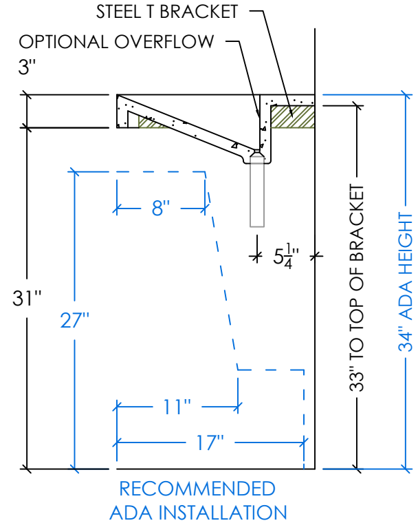
RIGHT SECTION
