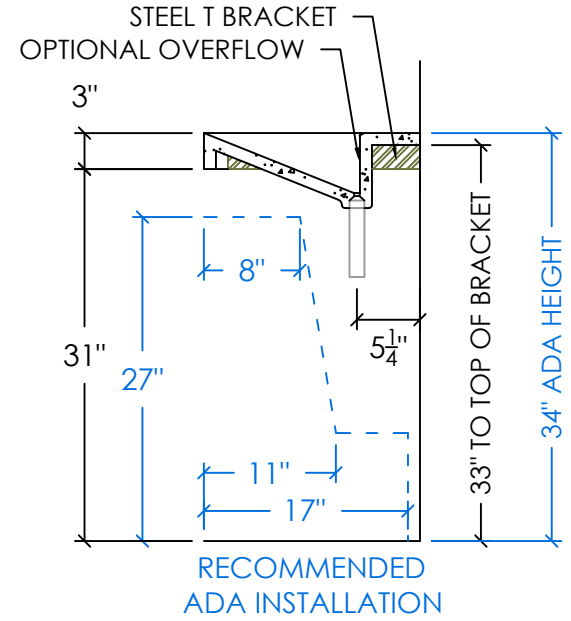
RIGHT SECTION
