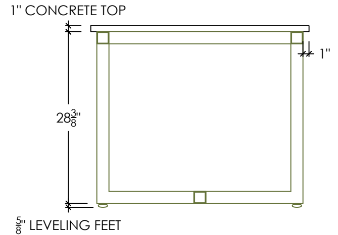
SIDE SECTION
