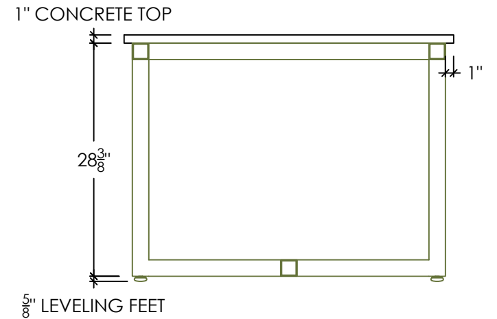
SIDE SECTION
