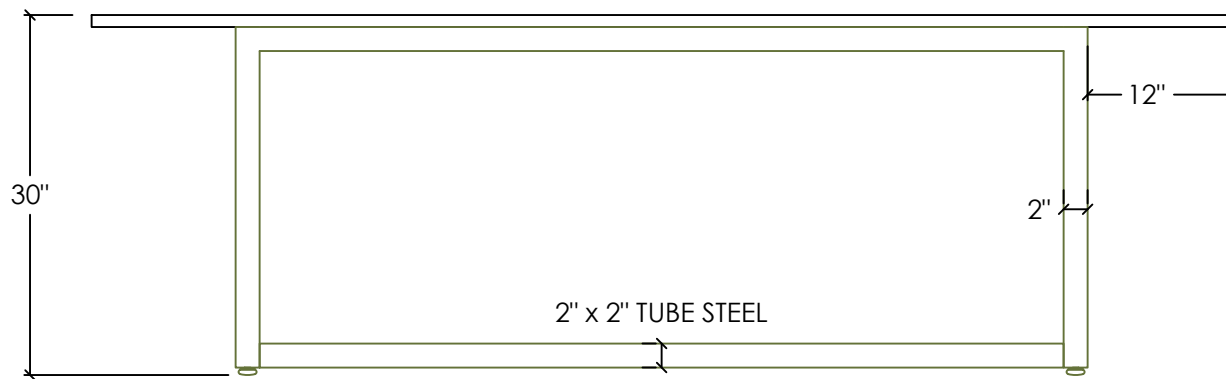
FRONT ELEVATION
