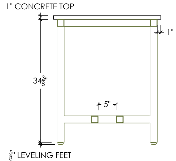
SIDE SECTION
