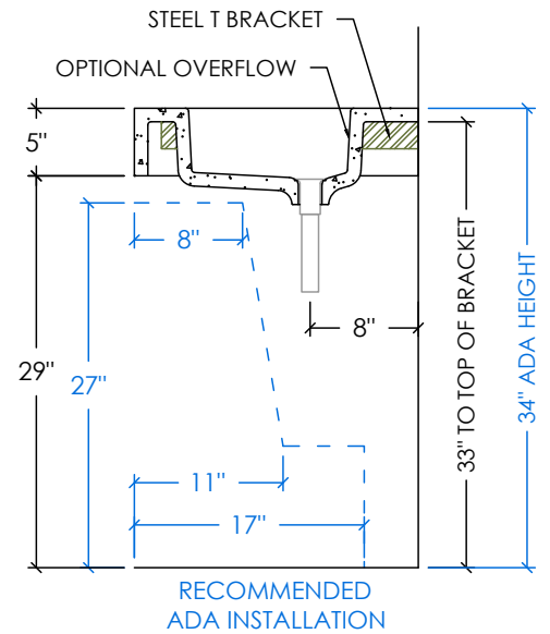
RIGHT SECTION
