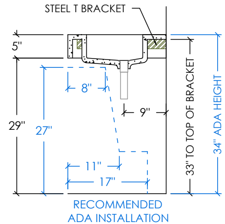
RIGHT SECTION
