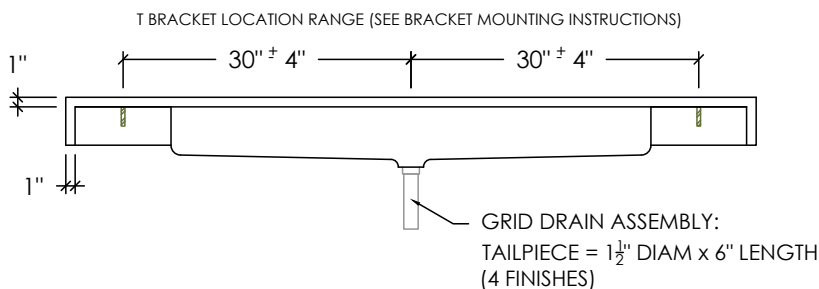
REAR ELEVATION
