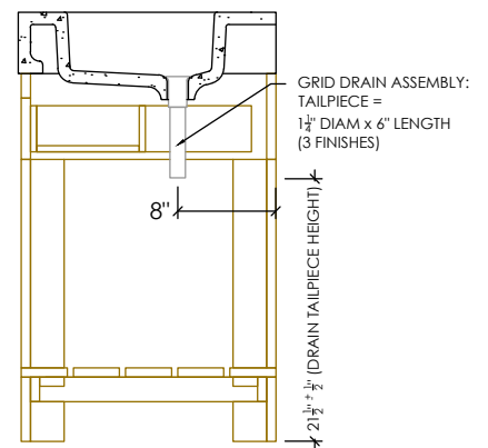
SECTION VIEW
